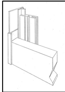
Panel Edge with Batten
