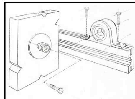
Panel Face Fastener
