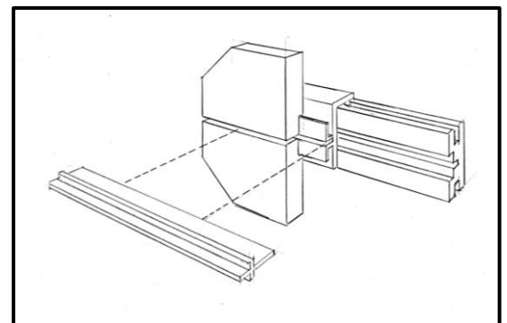
Panel Clip with Rib Insert
