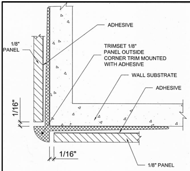
Outside Corner Profile
