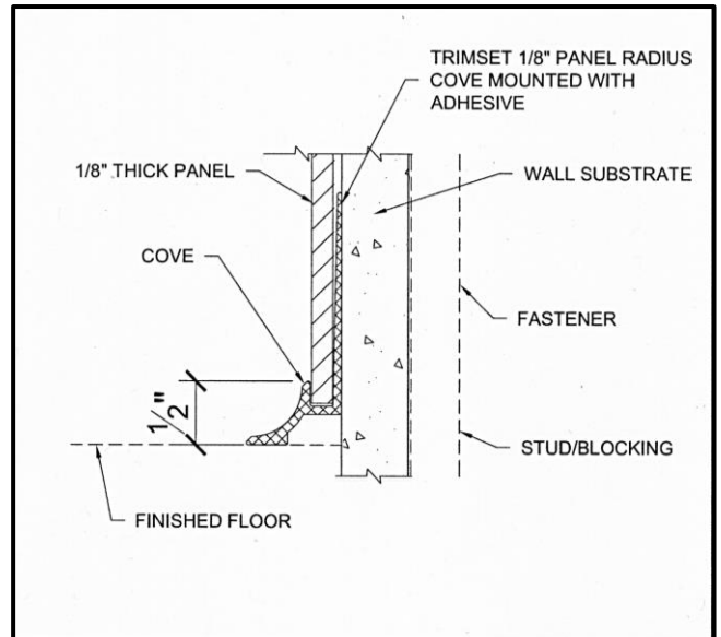
Base Cove Profile
